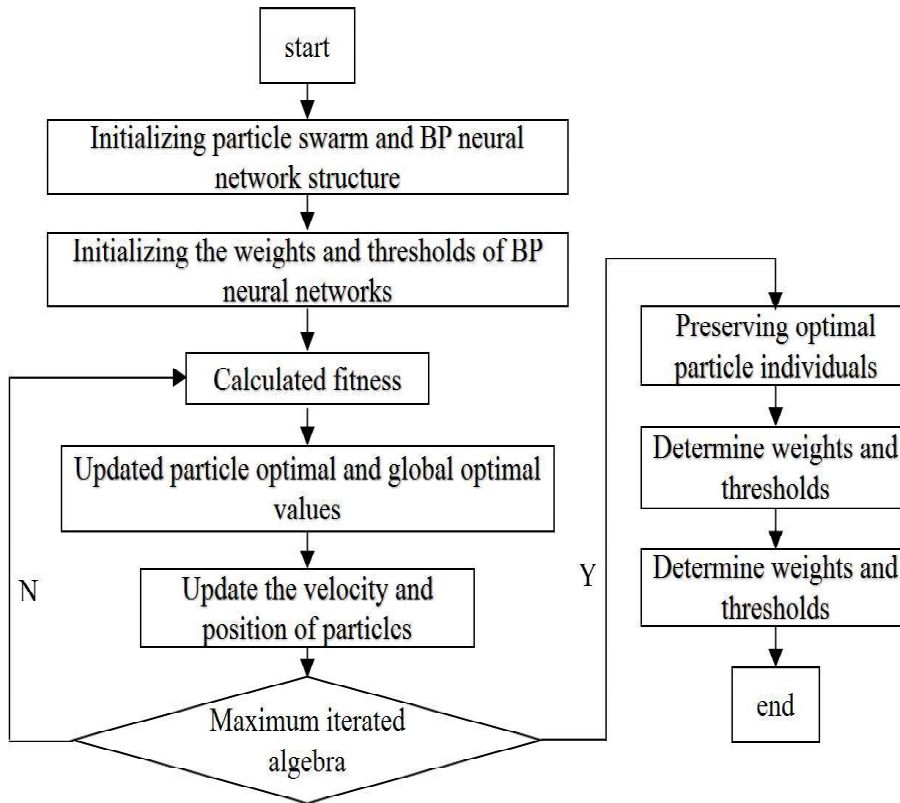
Figure 5. Flow Chart of Particle Swarm Optimization Bp Algorithm
