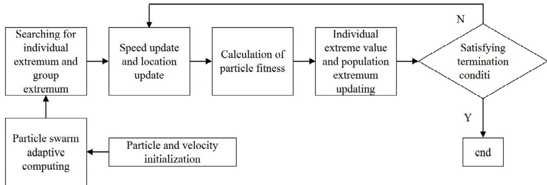
Figure 1. Flow chart of particle swarm optimization algorithm
