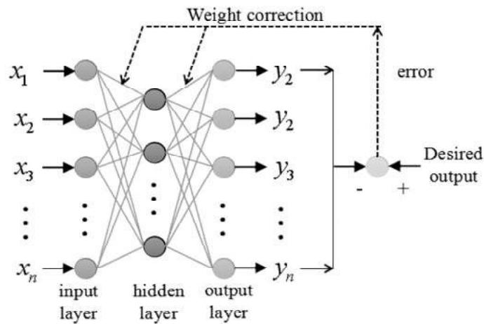
Figure 4. Structure of BP neural network
