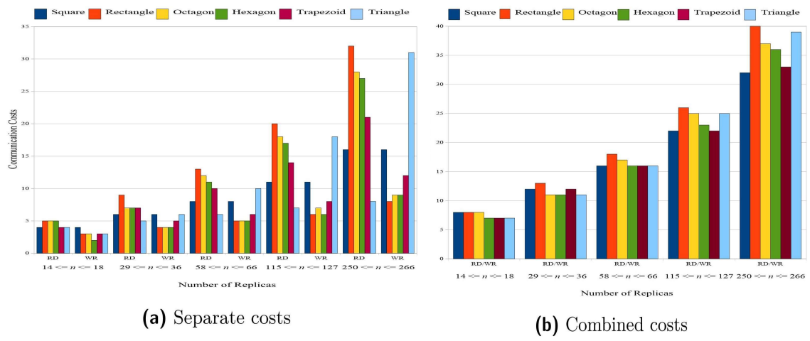
Figure 3. The communication costs of read (RD) and write (WR) operations
