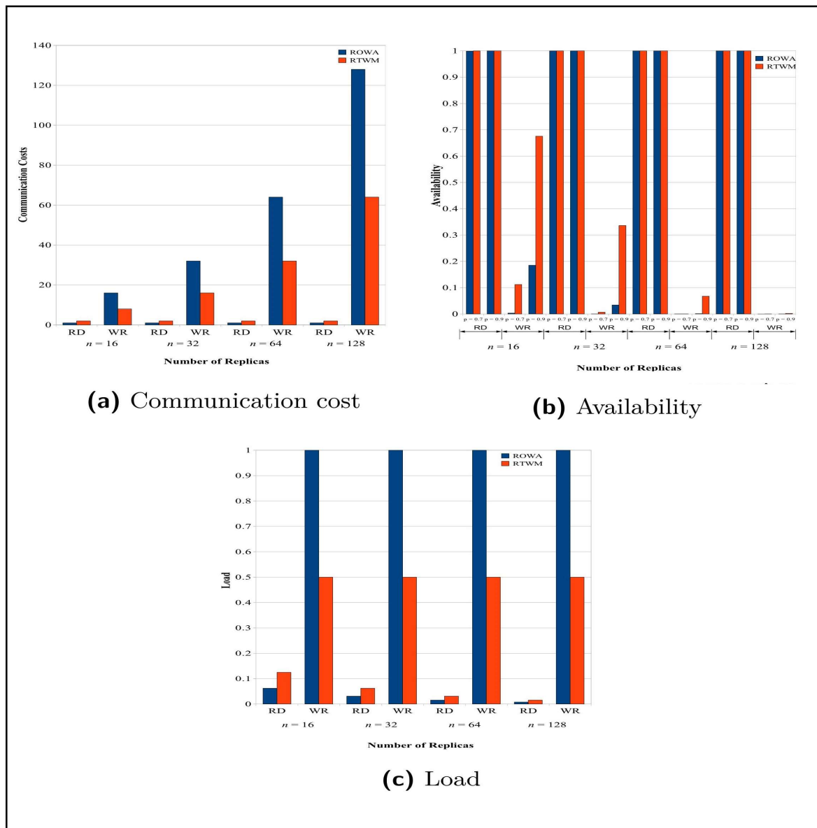
Figure 5. The RTWM vs ROWA protocols
