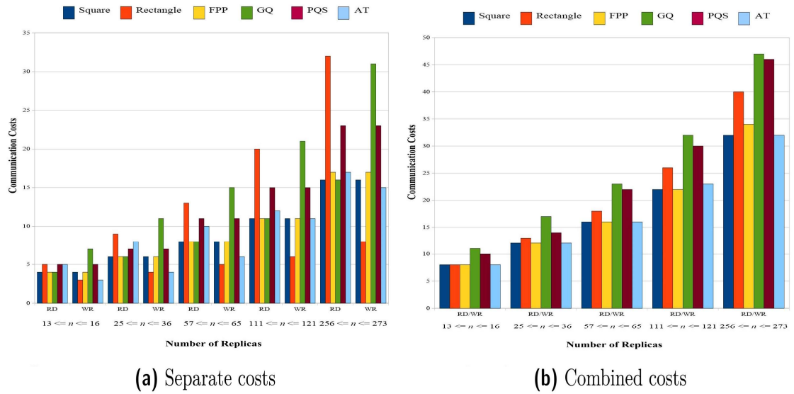
Figure 6. The communication costs of read (RD) and write (WR) operations
