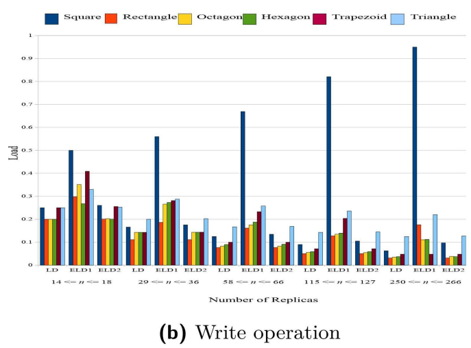
Figure 4. The system (LD) and expected system (ELD) loads for p = 0.7 and p = 0.9
