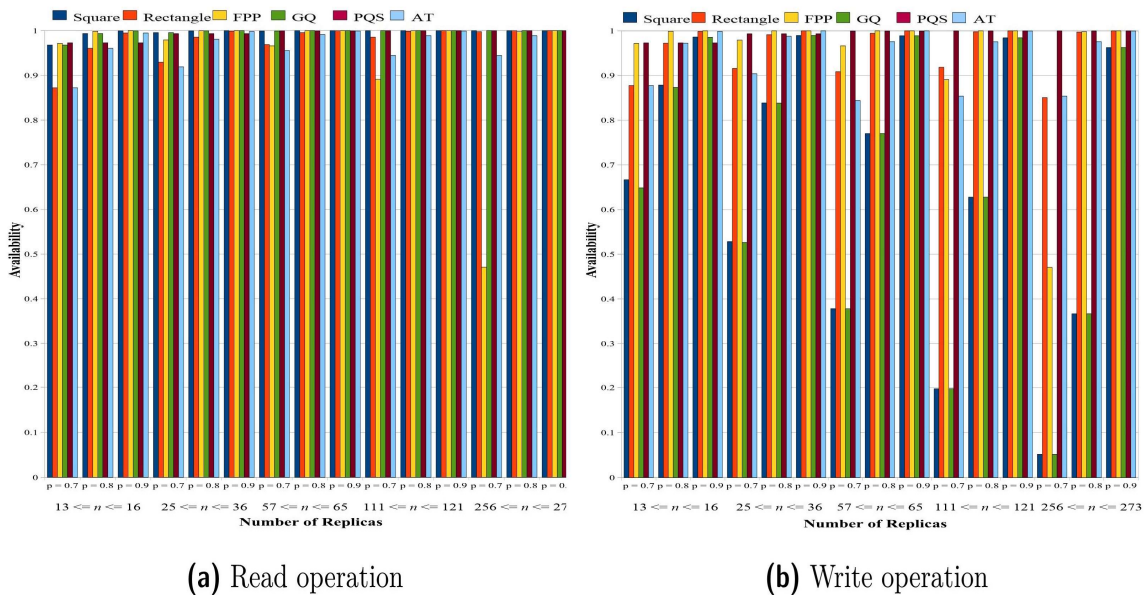
Figure 7. The availability of the operations for p = 0.7, 0.8 and 0.9
