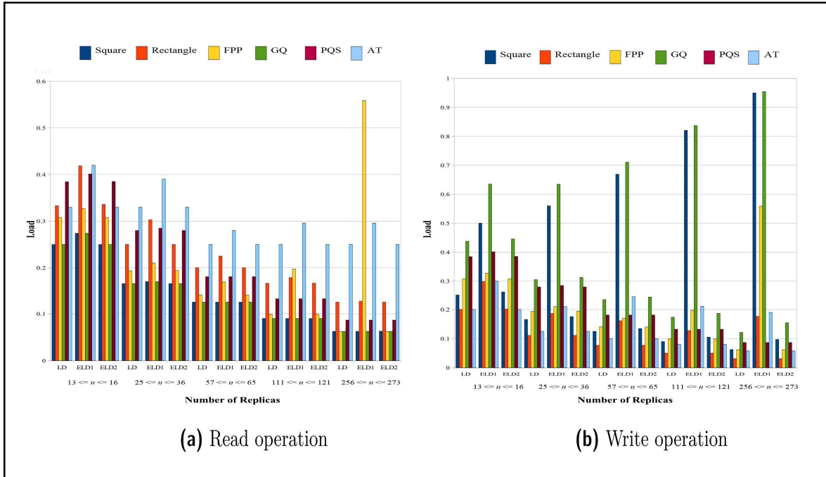
Figure 8. The system (LD) and expected system (ELD) loads for p = 0.7 and p = 0.9
