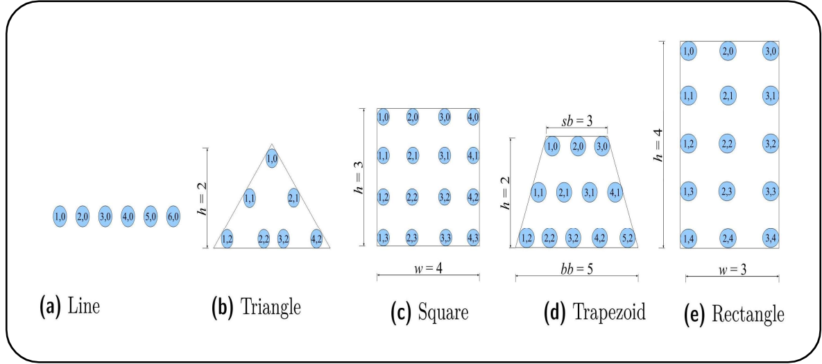
Figure 1. An Example of our basic Structures for n = 6, 7, 16, 12 and 15 Replicas Respectively
